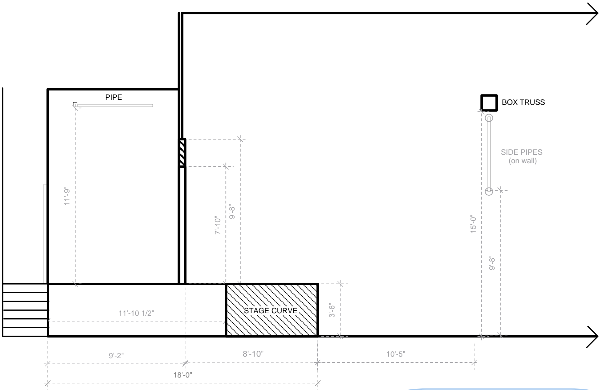
WONDER BALLROOM LONGITUDINAL SECTION scale 1/4" = 1'
